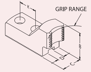
BAR GRIPPING
