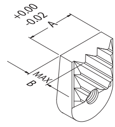
Angular
