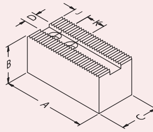
TYPE: AS-STEEL
