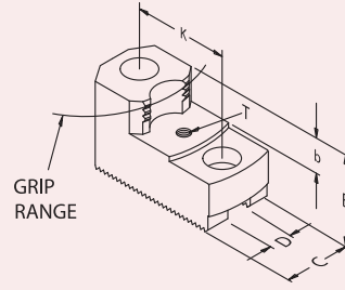
INTERNAL GRIP
