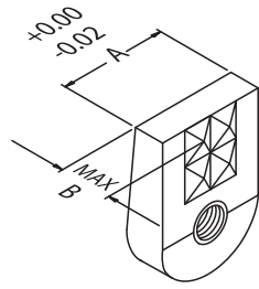
4 Point
