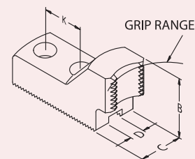
BAR GRIPPING
