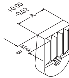
Straight
