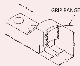
BAR GRIPPING
