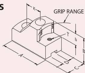
EXTERNAL GRIP
