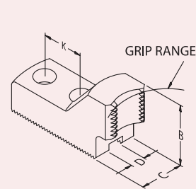
BAR GRIPPING
