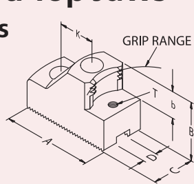
EXTERNAL GRIP
